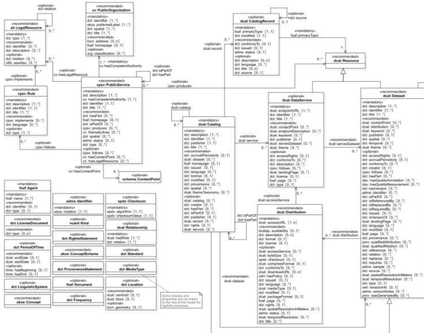
Fig. 2. Simplified UML class diagram showing the main relations between classes
